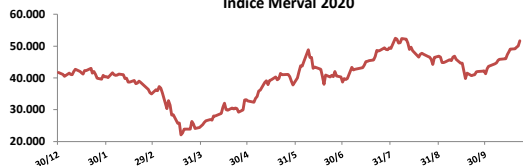
Indice Merval 2020
